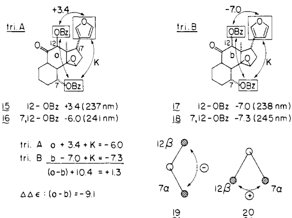
Figure 2. Deduction of 12-benzoate configurations.
